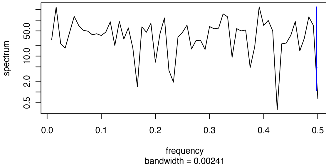
Unsmoothed periodogram
