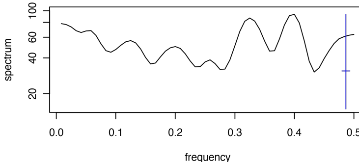
Smoothed periodogram
